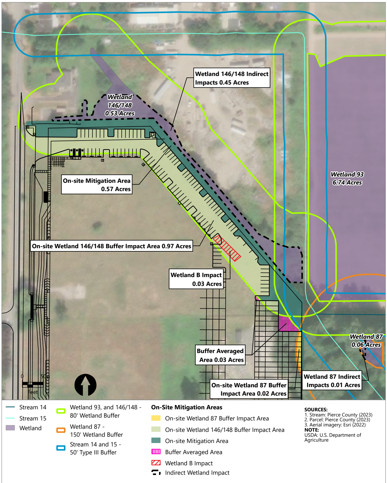
FIGURE 4: Conceptual On-Site Mitigation Plan - Freeman Road Logistics Project
